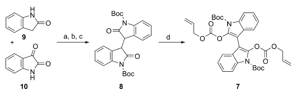
Scheme 2. Synthesis of dienol carbonate 7 . Reagents and conditions: a) HCl, HOAc, reflux, 82%; b) Boc 2 O, DMAP, NEt 3 , THF, 0°C → RT, 89%; c) 10 wt % Pd(OH) 2 /C, EtOH, RT, 96%. d) allyl chloroformate, NEt 3 , THF, 0°C → RT, 90%. DMAP = 4-dimethylaminopyridine.
