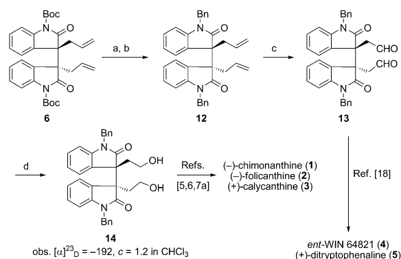
Scheme 3. Completion of the formal syntheses. Reagents and conditions: a) TFA, CH 2 Cl 2 , RT; b) NaH, DMF, 0 °C, then BnBr and warming to RT, 95 % over two steps; c) OsO 4 , NaIO 4 , 2,6-lutidine, dioxane/H 2 O, RT; d) NaBH 4 , MeOH, 0 °C, 52 % over two steps. DMF = N,N -dimethylformamide, TFA = trifluoroacetic acid.
